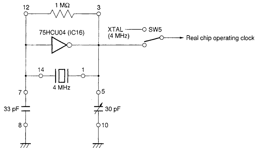
Figure 4-10. Peripheral Circuit of Component Block (PH1)
